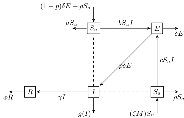
Fig. 2. A schematic diagram showing the dynamics of COVID-19 (Corona virus). The dotted lines represent contacts made by individuals in the respective classes and the solid lines show transfer from one class to another
