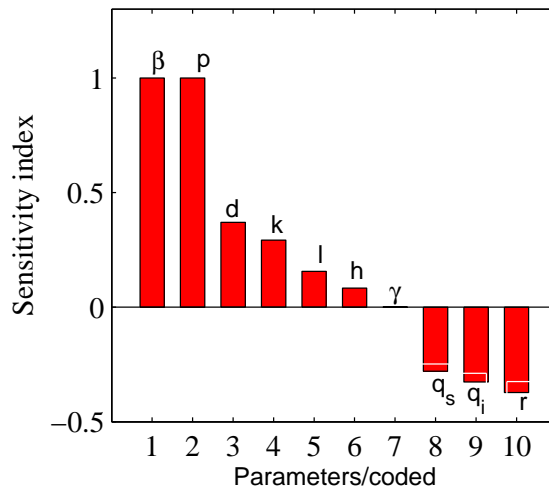
Fig. 3. Sensitivity analysis of different parameters on the basic reproduction number R_0
