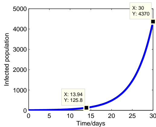
Fig. 1. The exponential projection of the number of infected individuals due to COVID-19 in Uganda without interventions (March, 2020)
