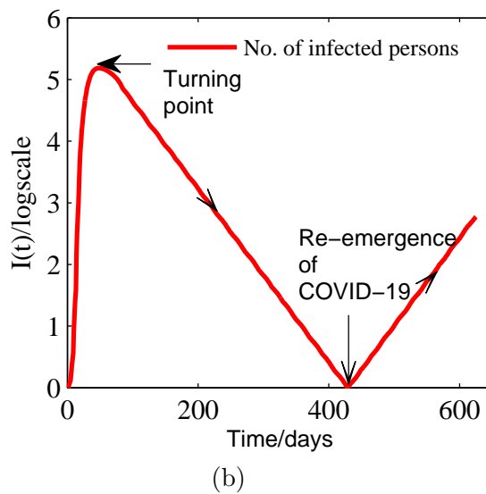
Fig .5(a) The number of infected persons as a function of time to linear scale. (b) The number of infected persons as a function of time to logarithm scale for R_0 = 0.46
