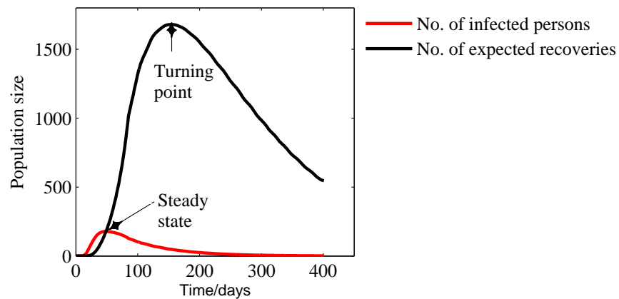
Fig. 4. Model (3.1) simulations for time series projection for the infected and expected recovered persons from COVID-19 in the presence of prevention and control measures.
